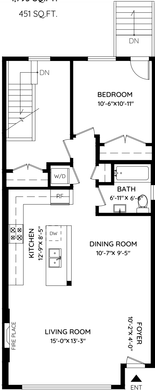
MAIN FLOOR 894 SQ.FT. CH: 8'-0"
