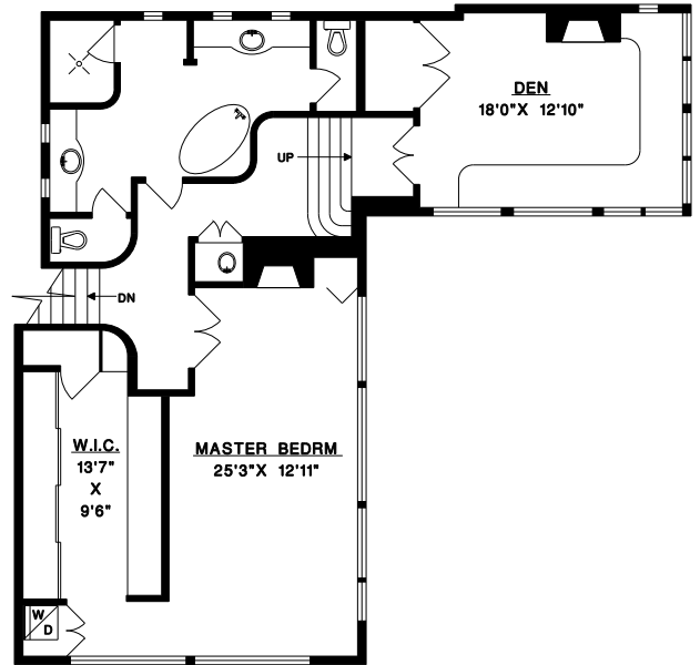
UPPER FLOOR
